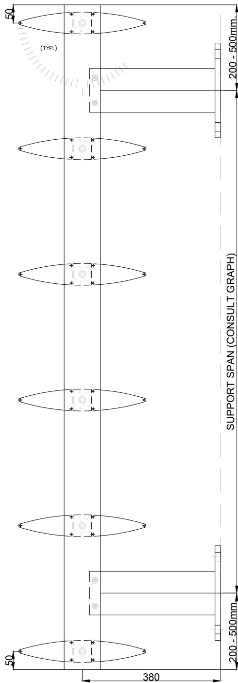
FIXED SYSTEM ON STRIP
